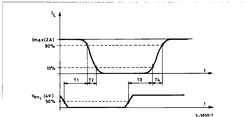
Figure 3 : Source Current Delay Times vs. Input or Enable Switching.
