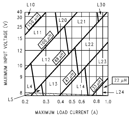
FIGURE 4. LM2672-3.3
