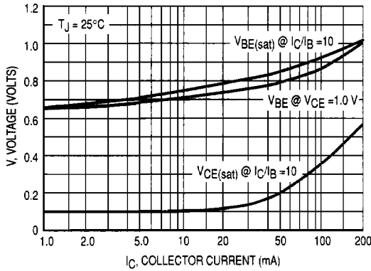
Figure 17. "ON" Voltages
