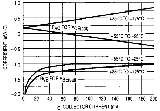
Figure 18. Temperature Coefficients
