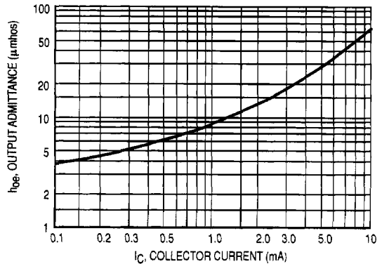
Figure 12. Output Admittance
