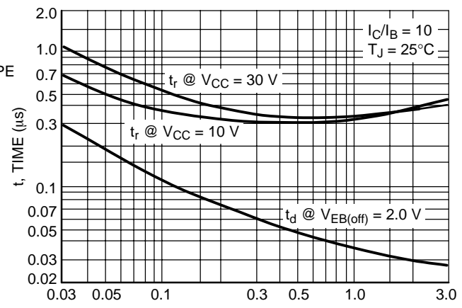
Figure 3. Turn-On Time
