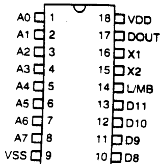
HT12A -18 DIP
