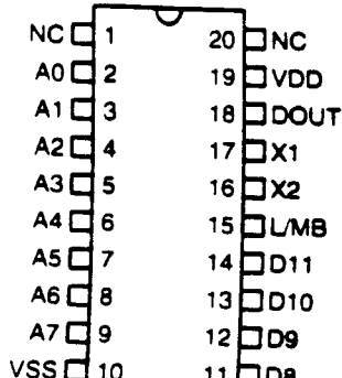
HT12A -20 SOP
