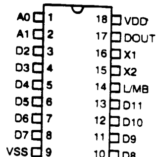
HT12C -18 DIP
