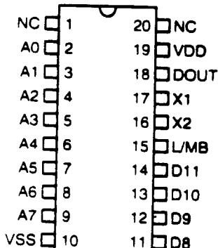
HT12B -20 SOP
