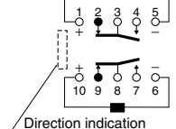
2-coil latching
