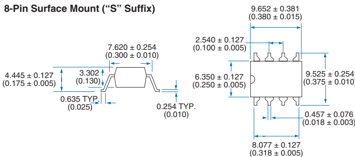
8-Pin Surface Mount ("S" Suffix)
