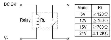
(c) Relay
