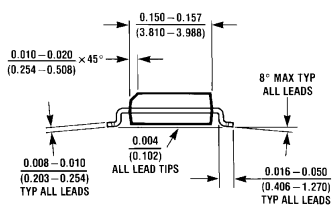
8-Lead (0.150" Wide) Molded Small Outline Package, Order Number LM2594M-3.3, LM2594M-5.0, LM2594M-12 or LM2594M-ADJ JEDEC NS Package Number M08A
