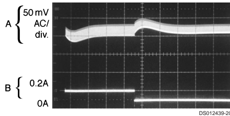
A: Output Voltage, 50 mV/div. (AC) B: 100 mA to 200 mA Load Pulse
