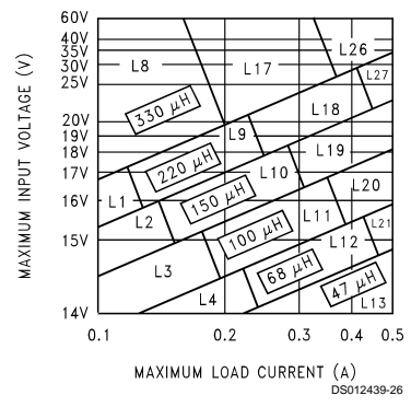
FIGURE 6. LM2594/LM2594HV-12
