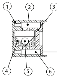
CROSS SECTION
