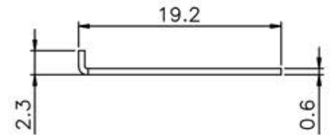
Fixing Washer
