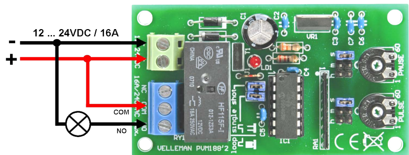
CONNECTION EXAMPLE: LOW VOLTAGE (12 ... 24VDC)
