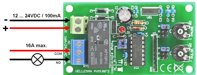
CONNECTION EXAMPLE: AC POWER
