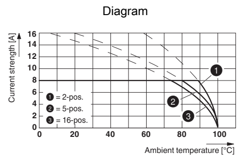
Type: FRONT-MC 1,5/...-ST-3,81 with SMC 1,5/...-G-3,81
