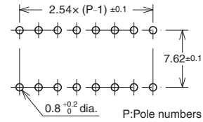
Dimensions of PCB pad (Top View)
