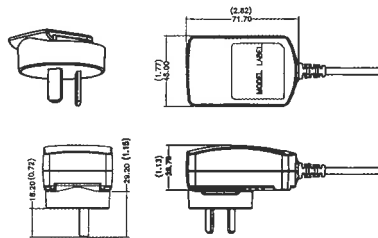
ASSEMBLY FROM HOUSING AND ARGENTINA CLIP
