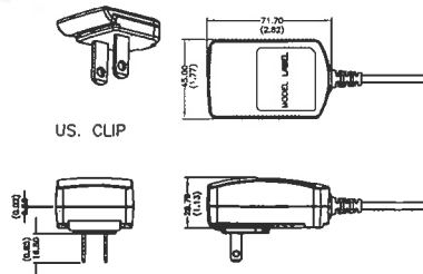
ASSEMBLY FROM HOUSING AND US. CLIP
