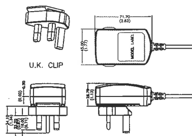
ASSEMBLY FROM HOUSING AND U.K. CLIP
