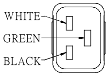
IEC-60320-C19
