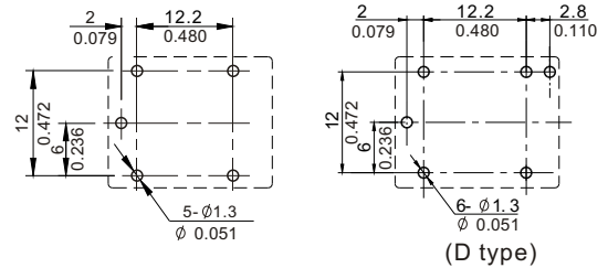
Mounting (Bottom view)
