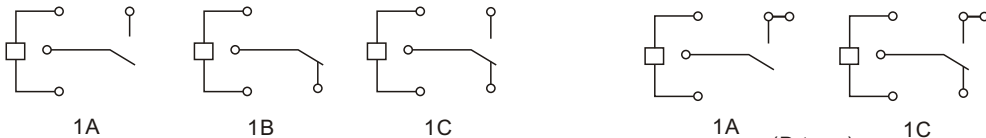
Wiring diagram (Bottom view)
