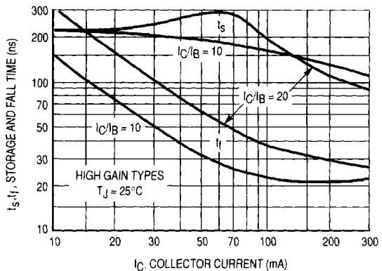
Figure 13. Turn-Off Behavior
