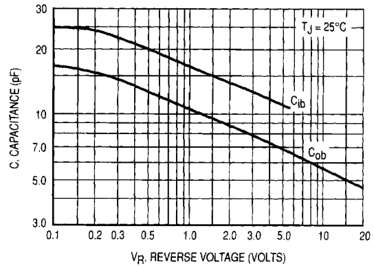
Figure 9. Capacitances
