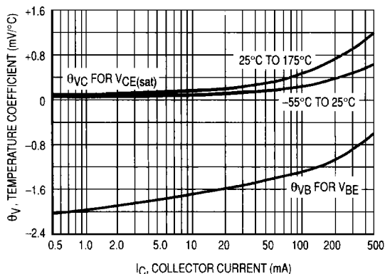
Figure 5. Temperature Coefficients
