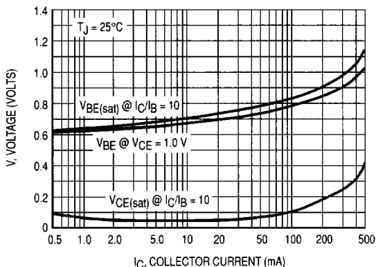
Figure 4. "ON" Voltages
