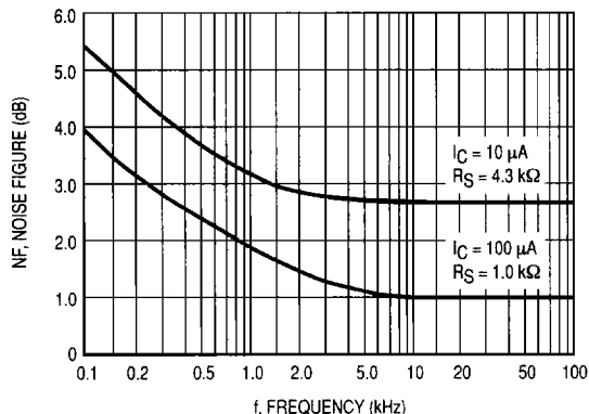
Figure 6. Frequency Effects
