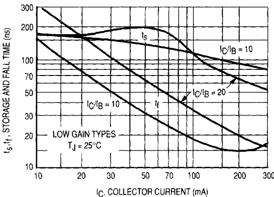
Figure 12. Turn-Off Behavior
