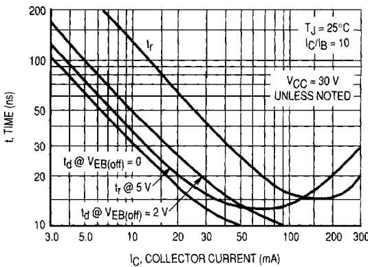
Figure 10. Turn-On Time
