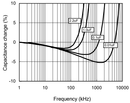
Frequency Characteristics
