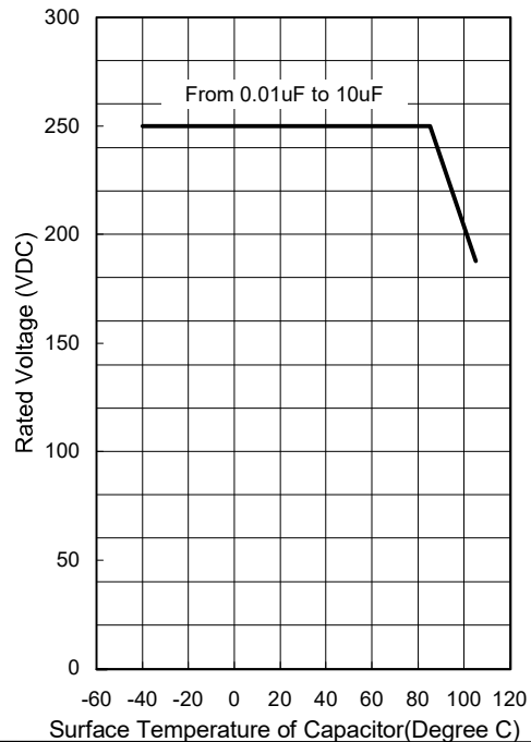
Voltage Derating by Temperature
