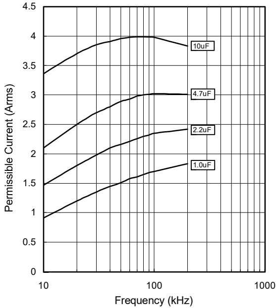
Permissible Current
