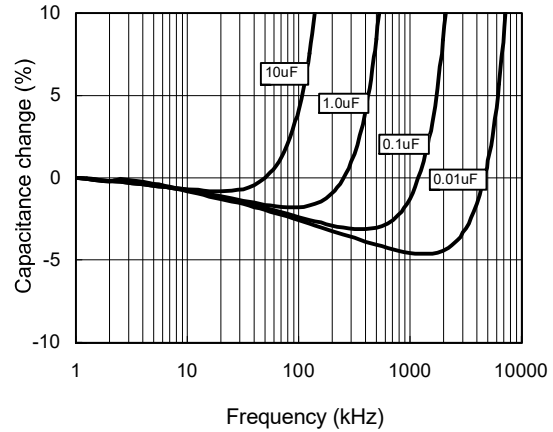
Frequency Characteristics
