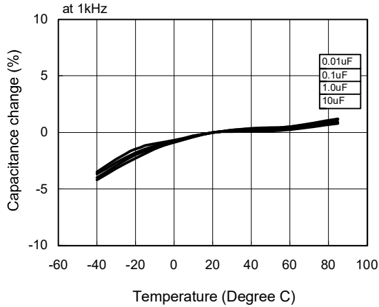
Temperature Characteristics
