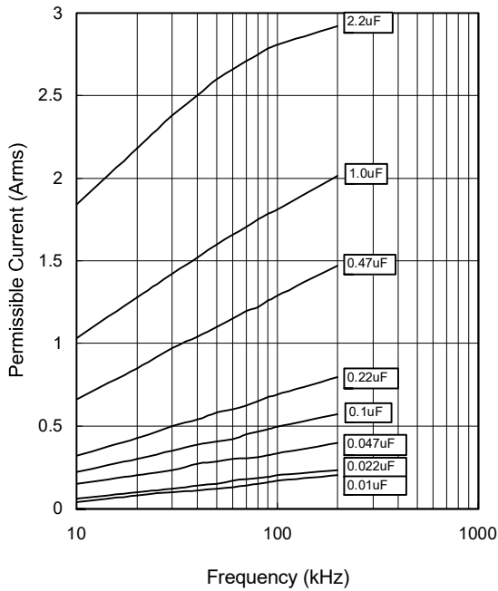
Permissible Current
