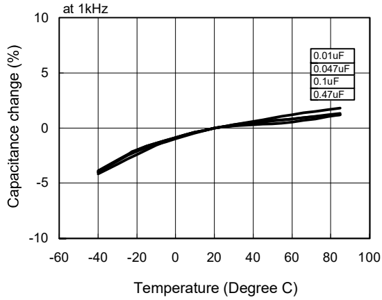
Temperature Characteristics
