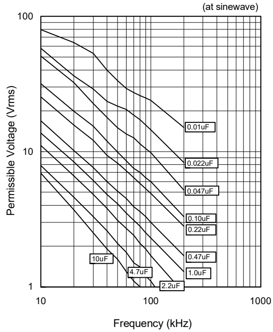
Permissible Voltage
