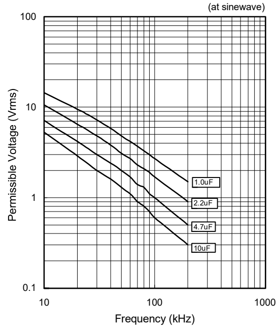
Permissible Voltage
