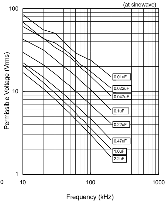
Permissible Voltage
