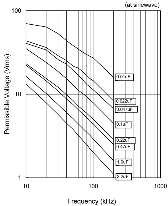
Permissible Voltage
