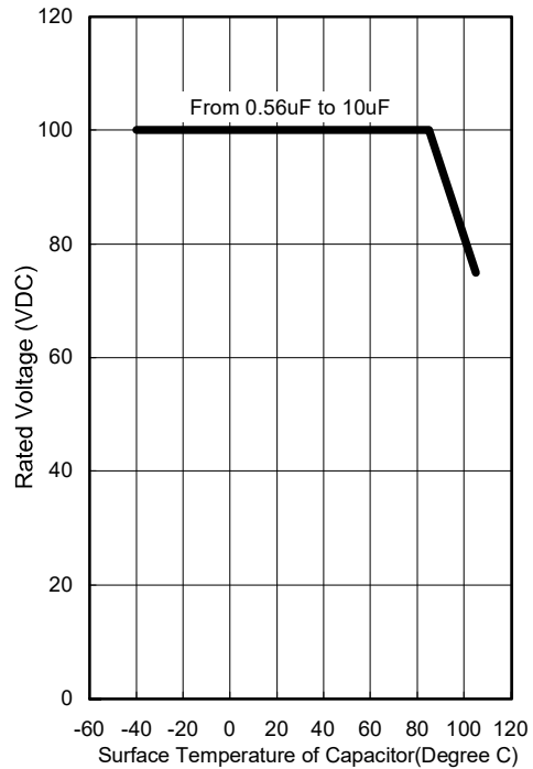
Voltage Derating by Temperature
