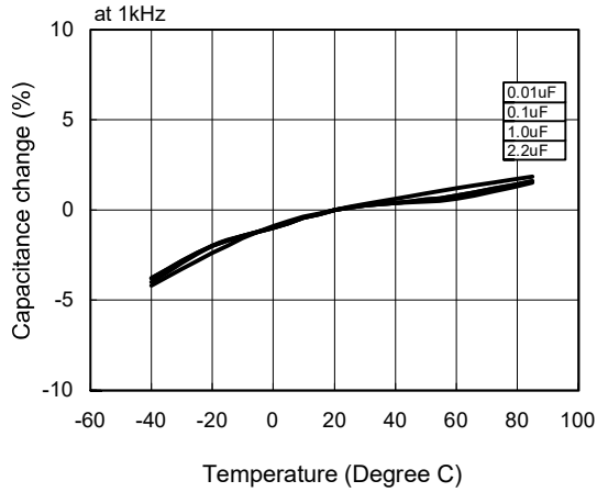
Temperature Characteristics
