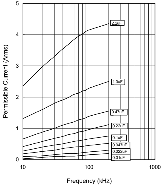
Permissible Current
