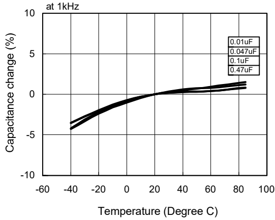
Temperature Characteristics
