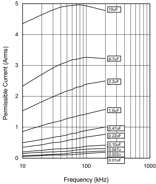
Permissible Current
