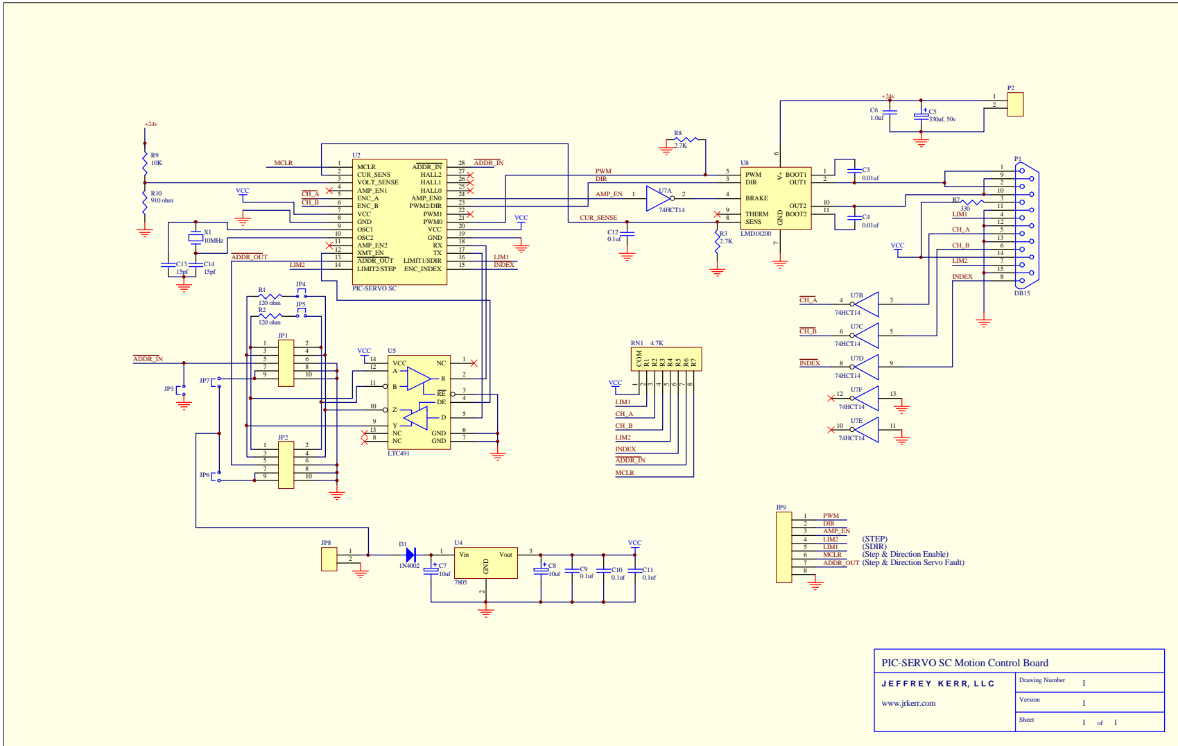
Figure 3 - PIC-SERVO SC Motion Control Board Schematic.
