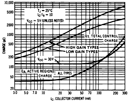
FIGURE 10 — CHARGE DATA
