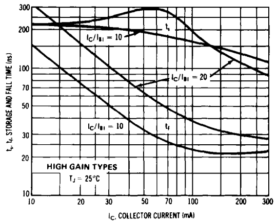
FIGURE 11 — TURN-OFF BEHAVIOR
