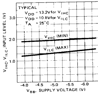
V IHC , V ILC INPUT LEVELS vs V BB SUPPLY VOLTAGE
