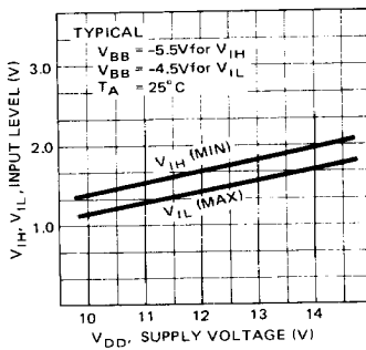
V IH , V IL INPUT LEVELS vs V DD SUPPLY VOLTAGE
