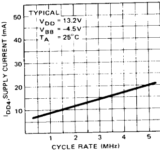
I DD4 (PAGE-MODE) vs CYCLE RATE
