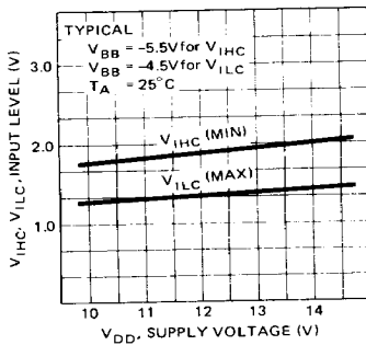
V IHC , V ILC INPUT LEVELS vs V DD SUPPLY VOLTAGE
