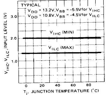
V IHC , V ILC INPUT LEVELS vs T J JUNCTION TEMPERATURE
