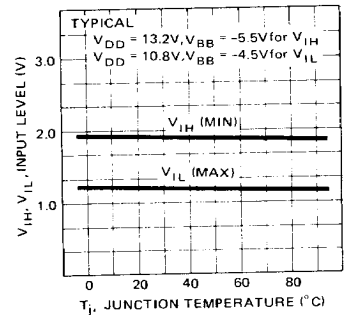
V IH , V IL INPUT LEVELS vs T J JUNCTION TEMPERATURE
