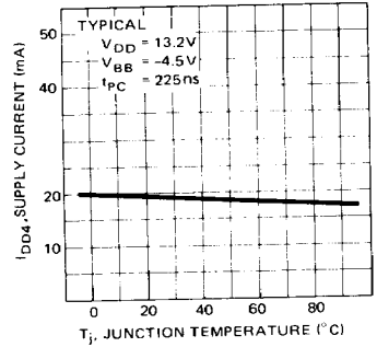
I DD4 (PAGE-MODE) vs T J JUNCTION TEMPERATURE
