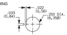
Without Locking Ring
