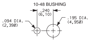
With Standard Locking Ring
