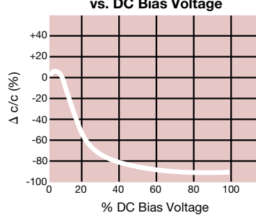
Capacitance Change vs. DC Bias Voltage
