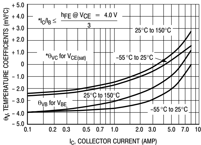
Figure 11. Temperature Coefficients
