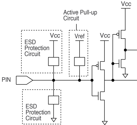
Typical Input
